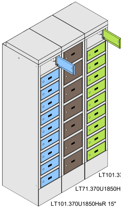
LT101.370U1850HsR 15"
